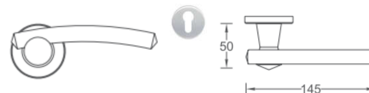
Marco Polo Stainless Steel Lever Handle on Rosette
